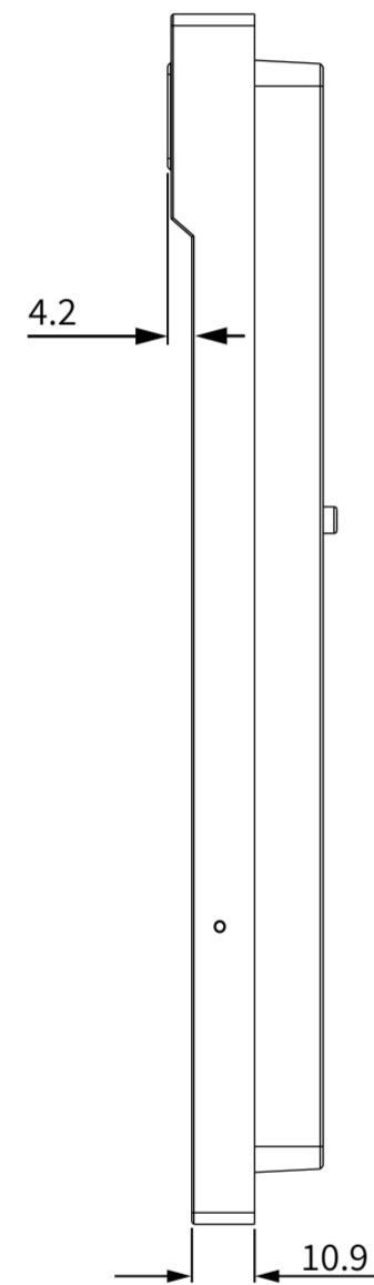
② RIGHT VIEW
