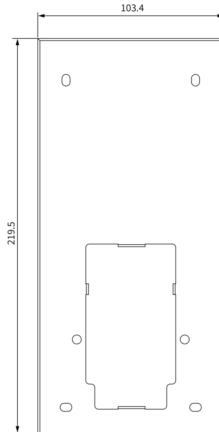
① FRONT VIEW
