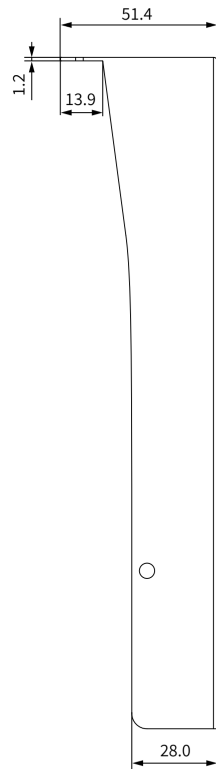
② RIGHT VIEW
