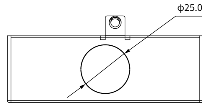
⑥ BOTTOM VIEW
