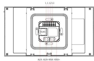
4 BACK VIEW
